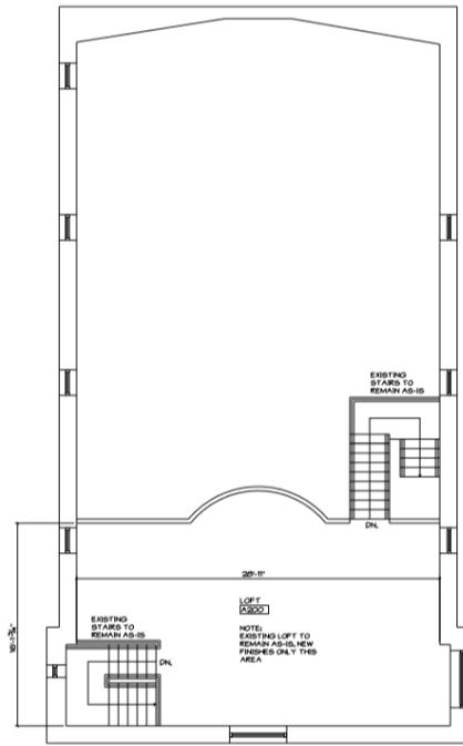
1 BALCONY PLAN
